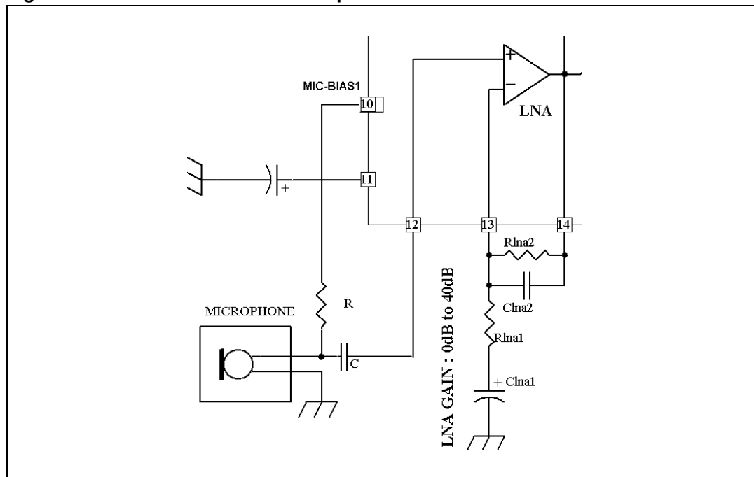
Figure 27. Electret condenser microphone source
