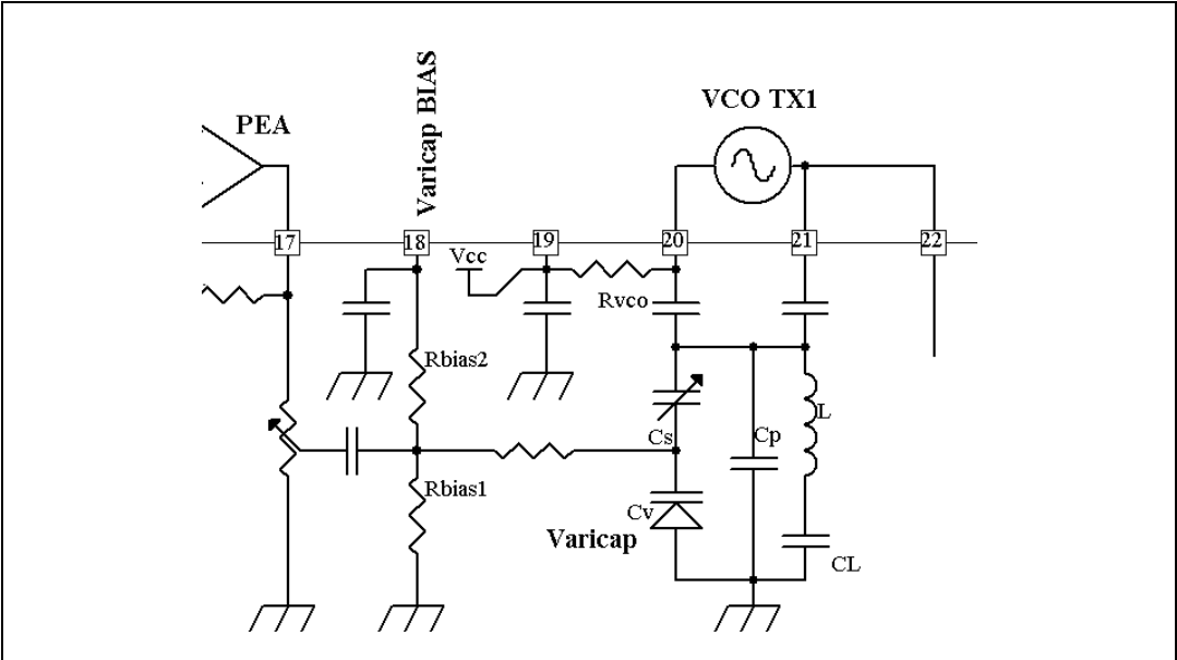
Figure 33. VCO schematics
