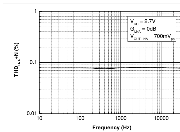
Figure 4. LNA distortion vs. frequency
