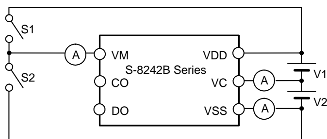
Figure 7 Test circuit 3
