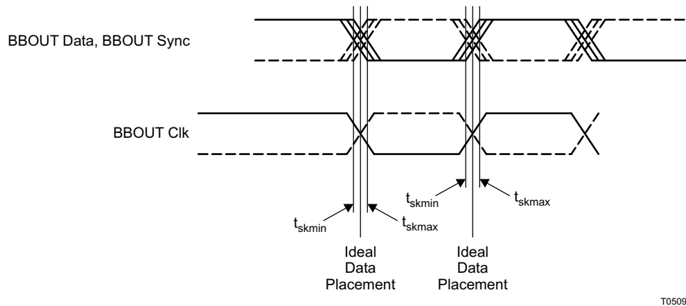
Figure 16. RX Baseband LVDS DDR0 Output Timing Specifications
