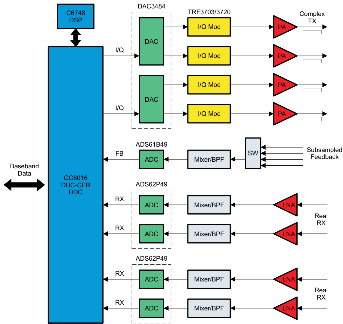
Figure 4. Four-Antenna-Mode Subsampled Real-Feedback Example Diagram
