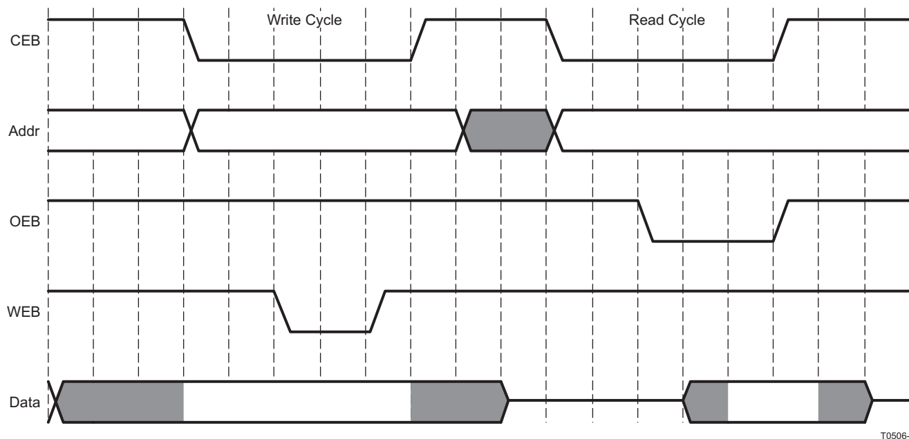
Figure 13. MPU Interface Format
