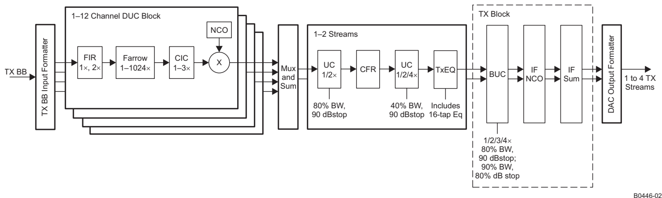
Figure 8. TX Functional Block Diagram
