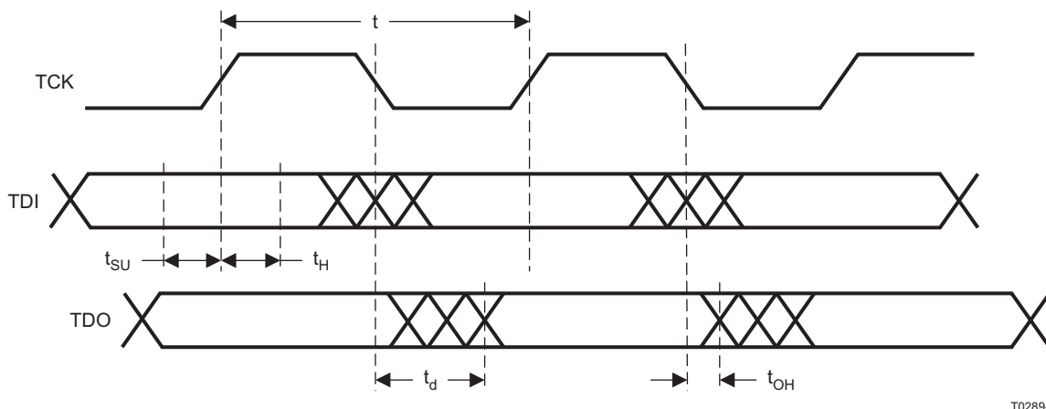
Figure 23. JTAG Timing Specifications
