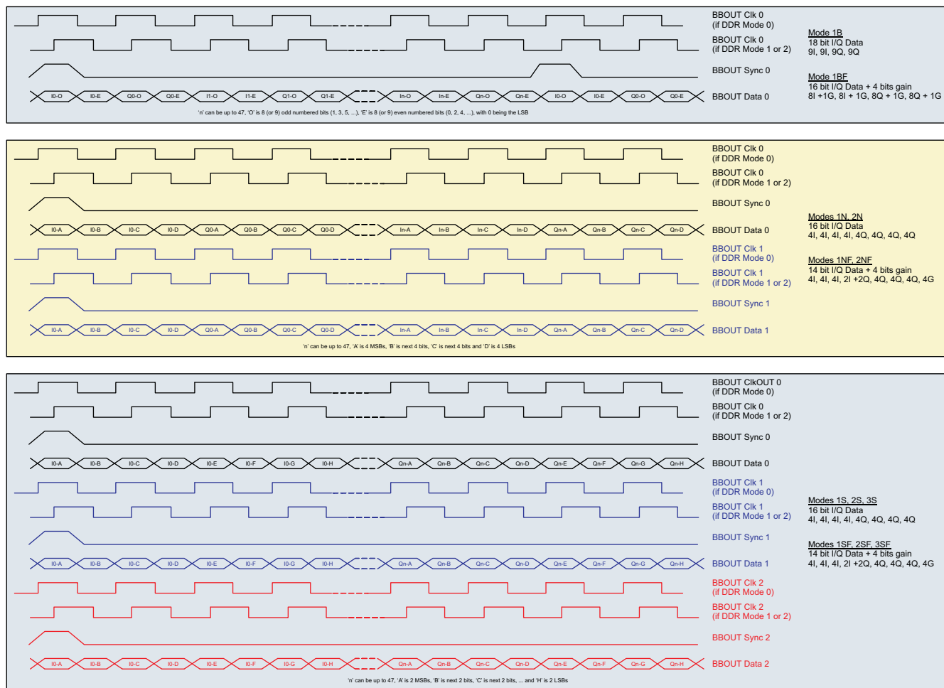
Figure 12. RX BB Formats
