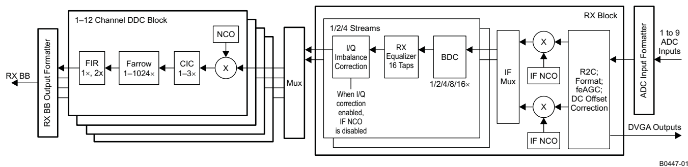
Figure 9. RX Functional Block Diagram
