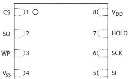
Figure 1.2 Pin Diagrams (Top View)
