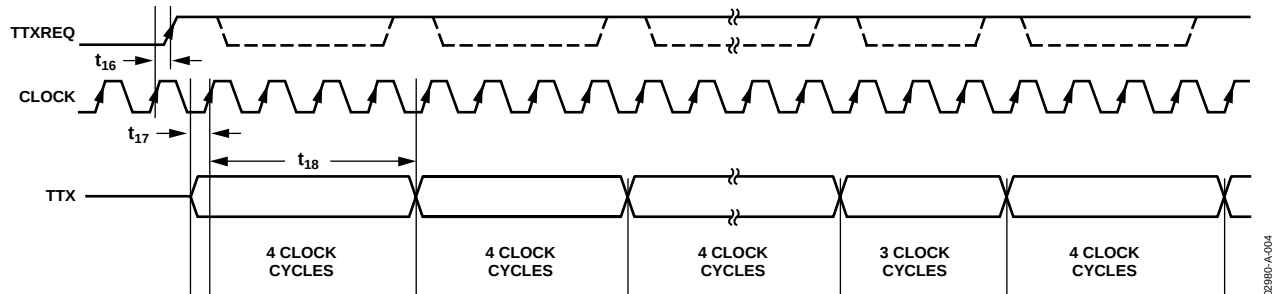
Figure 4. Teletext Timing Diagram
