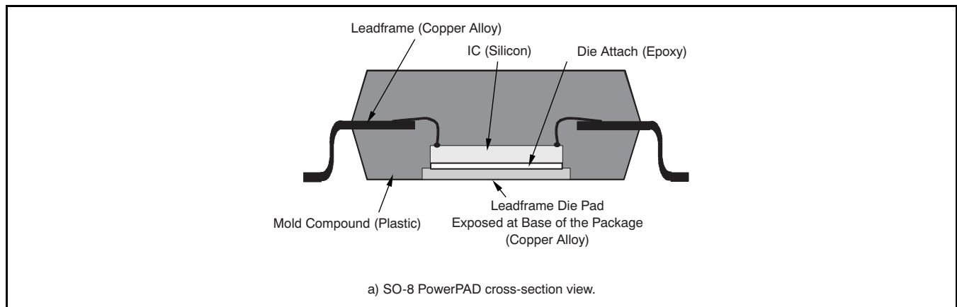
Figure 71. Cross-Section View of a PowerPAD Package
