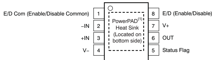
DDA PACKAGE SO-8 PowerPAD (TOP VIEW)
