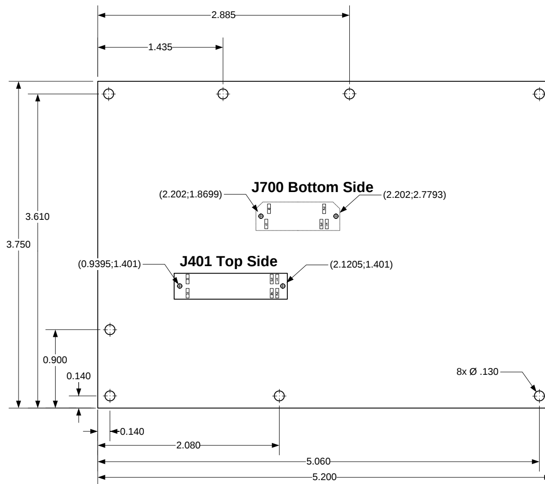
Figure 9: MityARM-335x Development Kit Outline, Mounting Hole Locations, Hirose DF9-41P-1V(32) expansion header J700 and Molex 87832-3420 LCD header J401 (Top View, inches)
