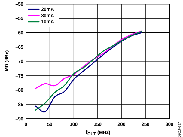
Figure 20. IMD vs. f_{OUT} over f_{SC} , 2× Interpolation, f_{DATA} = 250 MSPS, Digital Scale = 0 dBFS
