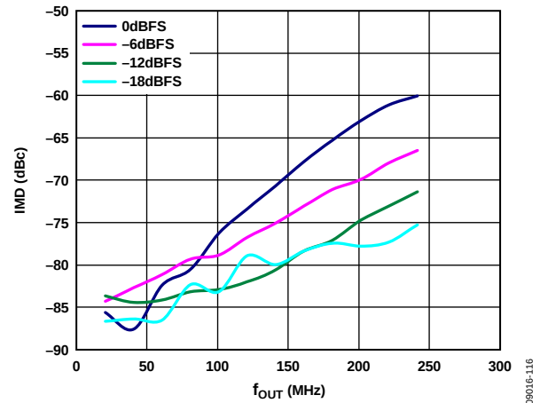
Figure 19. IMD vs. f_{OUT} over Digital Scale, 2× Interpolation, f_{DATA} = 250 MSPS, f_{SC} = 20 mA
