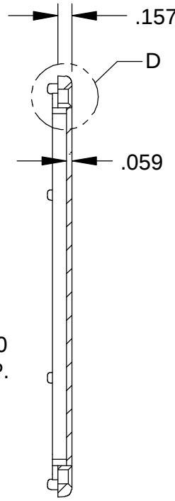
SECTION C-C
