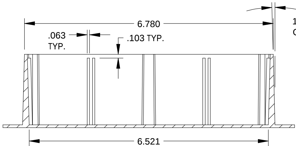
SECTION B-B
