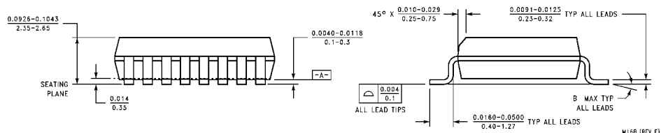
-B- 0.3977-0.4133 10.10-10.50 16 15 14 13 12 11 10 9 LEAD NO 1 IDENTIFICATION 0.2914-0.2992 7.4-7.6 -C- 0.3940-0.4190 10.00-10.65 1 2 3 4 5 6 7 8 0.0950 1.27 0.0138-0.0200 0.350-0.508 TYP 0.010 0.25 M A C S B
