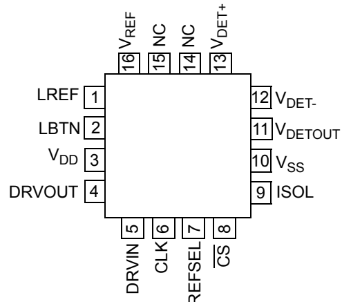
MCP2036 16-pin QFN
