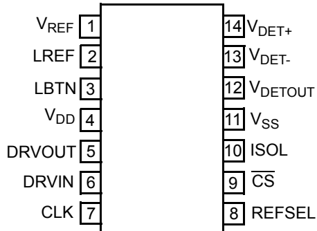
MCP2036 14-pin PDIP, SOIC
