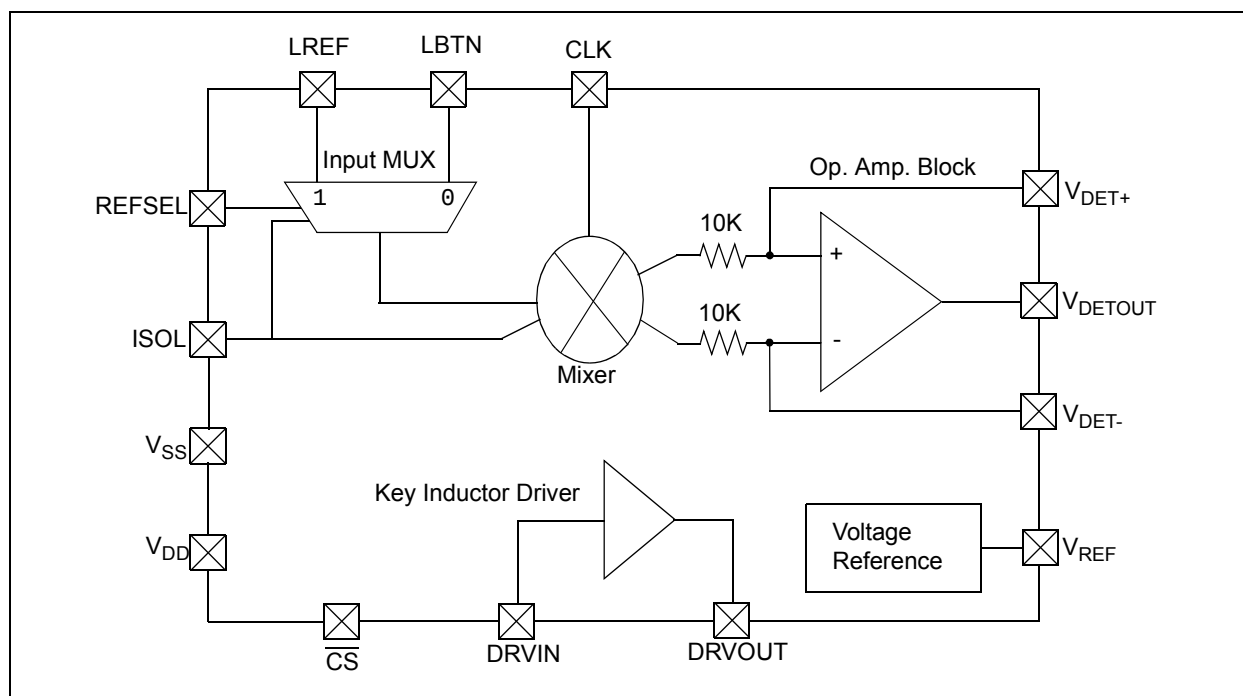
FIGURE 1-1: MCP2036 Block Diagram
