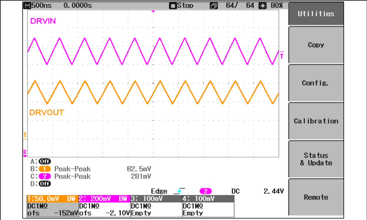
FIGURE 5-2: Inductor Driver Transfer Function (Rload = 100 Ohm)
