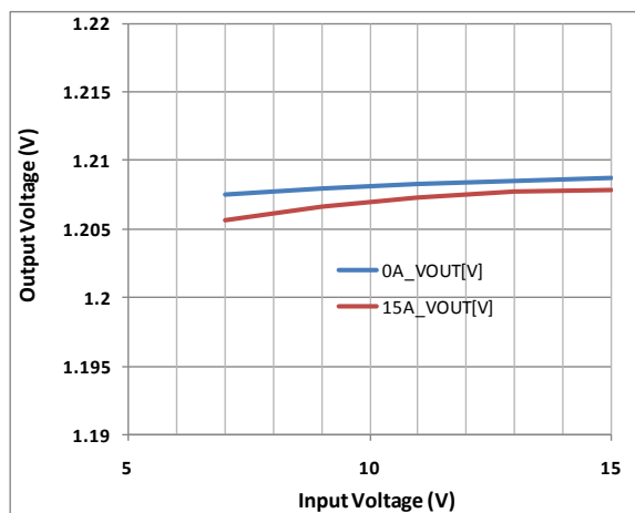
Figure 11. Line Regulation
