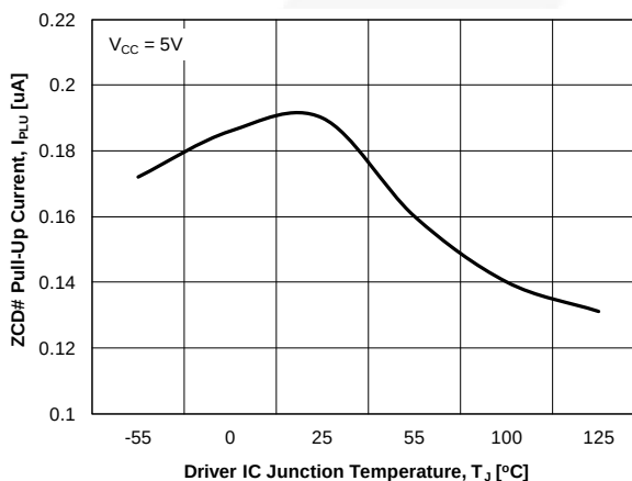
Figure 21. ZCD# Pull-Up Current vs. Temperature
