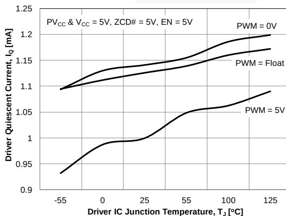
Figure 27. Driver Quiescent Current vs. Temperature
