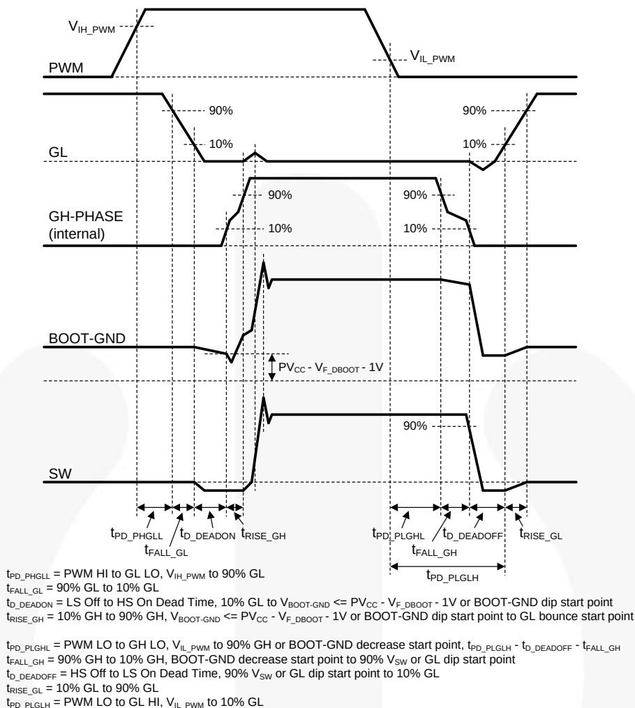
Figure 29. PWM Timing Diagram
