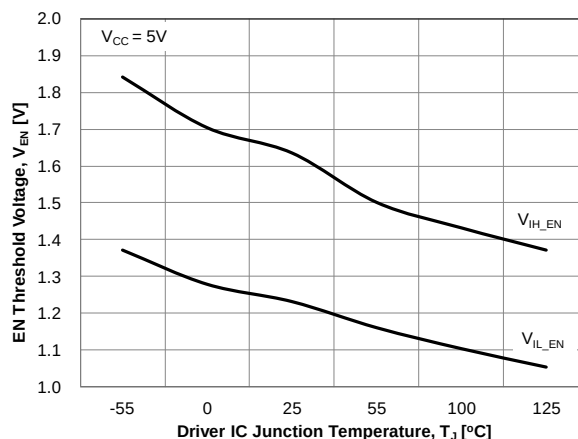
Figure 23. EN Threshold vs. Temperature
