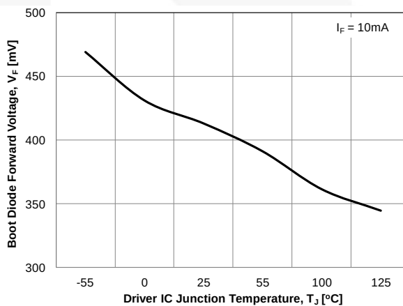
Figure 25. Boot Diode Forward Voltage vs. Temperature
