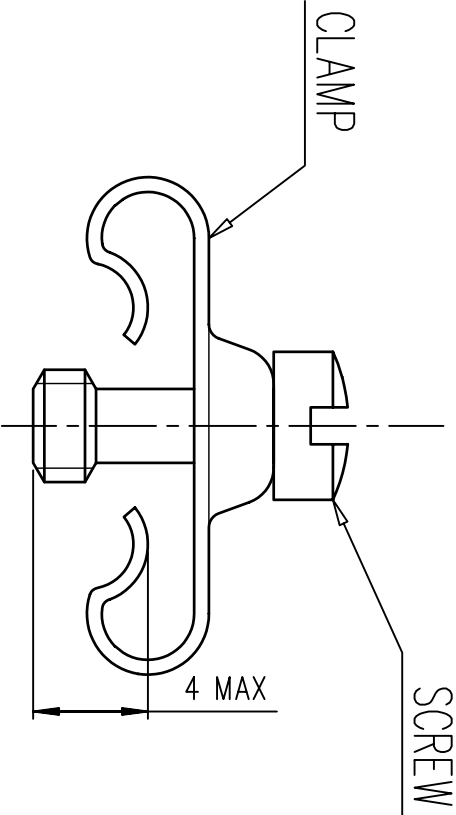
ASSEMBLY VIEW
