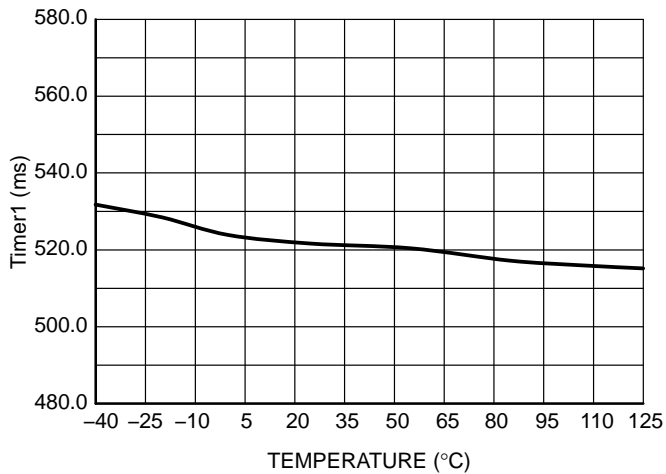
Figure 55. Fault Timer Duration – Overload, Timer1, C/D Version
