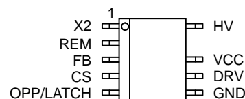
NCP1249A/B (Top View)
