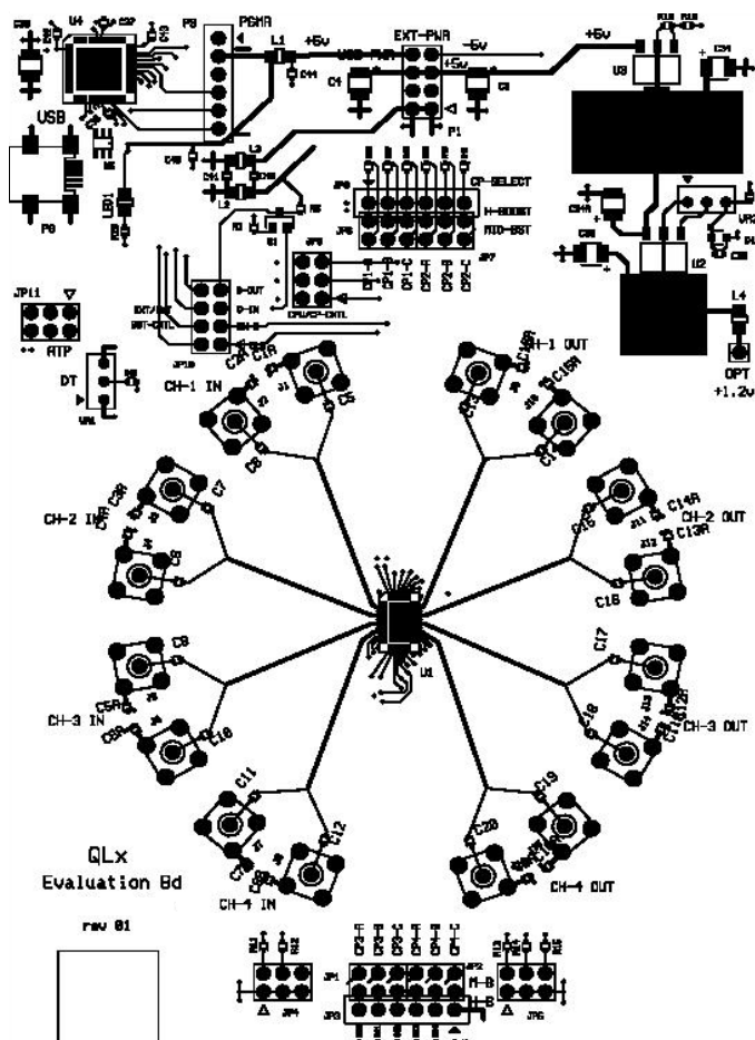
FIGURE 1. QLx4300-S45 EVALUATION BOARD PCB OUTLINE
