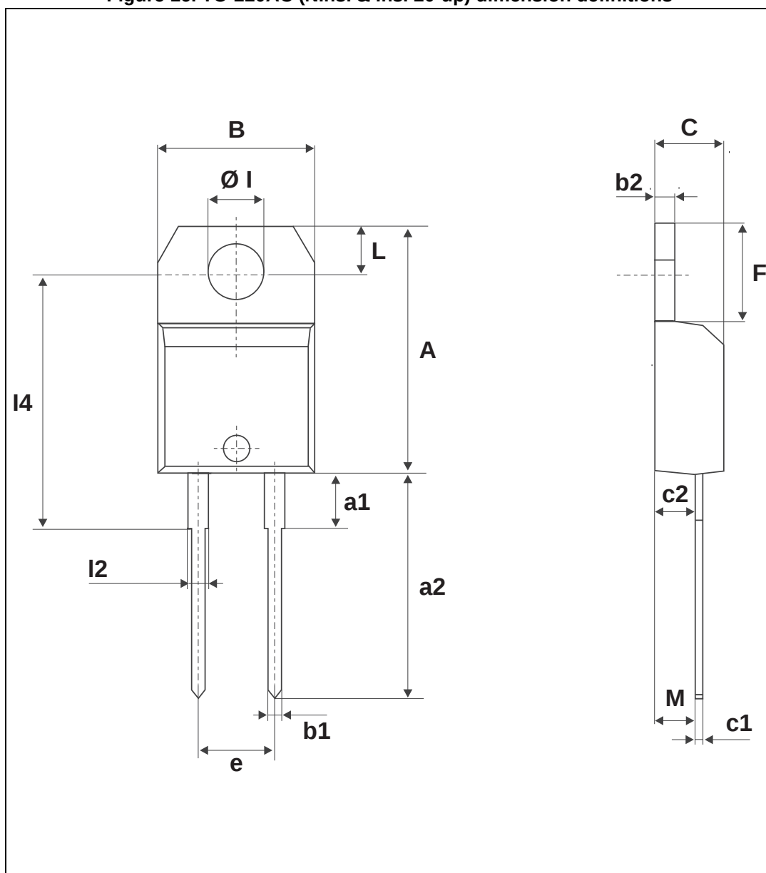
Figure 16. TO-220AC (NIns. &amp; Ins. 20-up) dimension definitions
