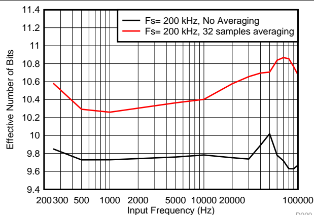
Figure 5-11. Effective number of bits vs Input frequency (Internal Reference, No Scaling)
