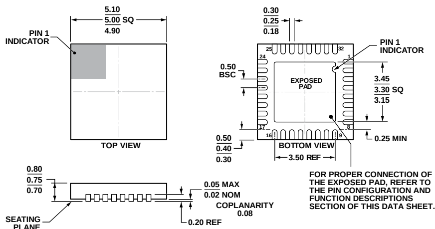
Figure 146. 32-Lead Lead Frame Chip Scale Package [LFCSP_WQ] 5 mm × 5 mm Body, Very Very Thin Quad (CP-32-13)
