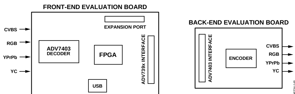
Figure 144. ADV7390/ADV7391/ADV7392/ADV7393 Front-End and Back-End Evaluation Boards
