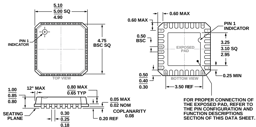
Figure 145. 32-Lead Lead Frame Chip Scale Package [LFCSP_VQ] 5 mm × 5 mm Body, Very Thin Quad (CP-32-2)
