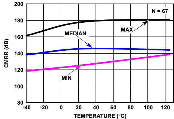
FIGURE 28. CMRR vs TEMPERATURE, V_{CM} = -2.5V TO +2.5V , V_+ = \pm 2.5V
