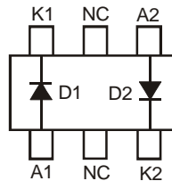
Internal Schematic
