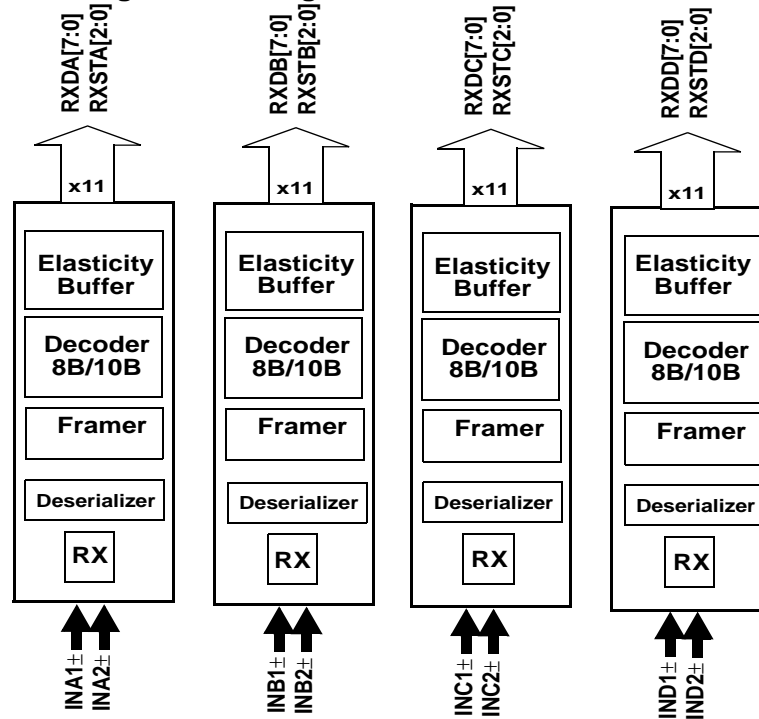
CYP15G0401RB Receiver Logic Block Diagram
