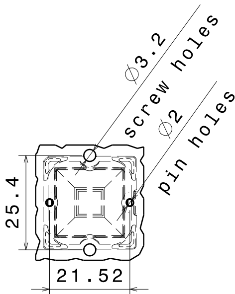
PCB-Suggestion
