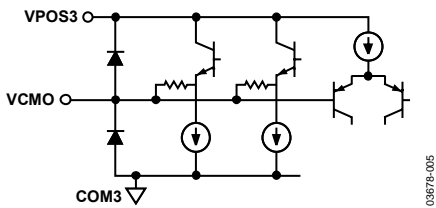
Figure 5. Circuit C
