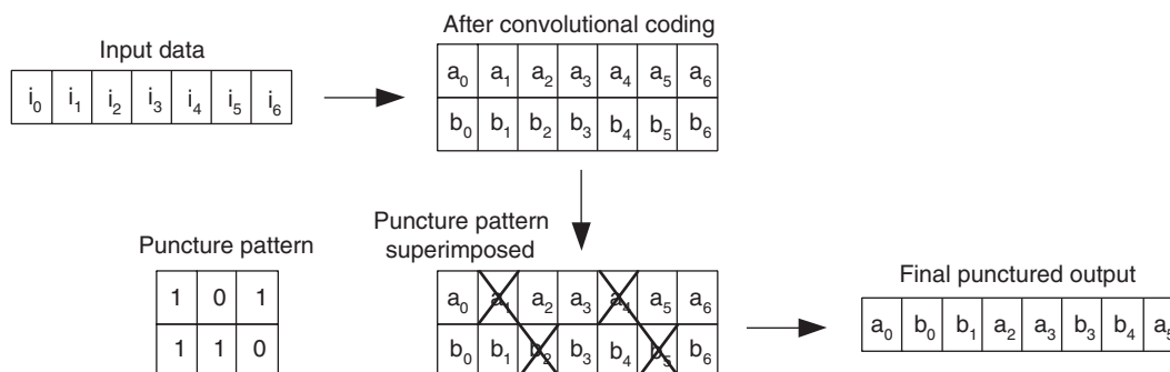
Figure 3. Puncturing Process
