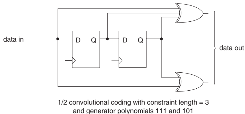
Figure 2. Convolutional Encoding
