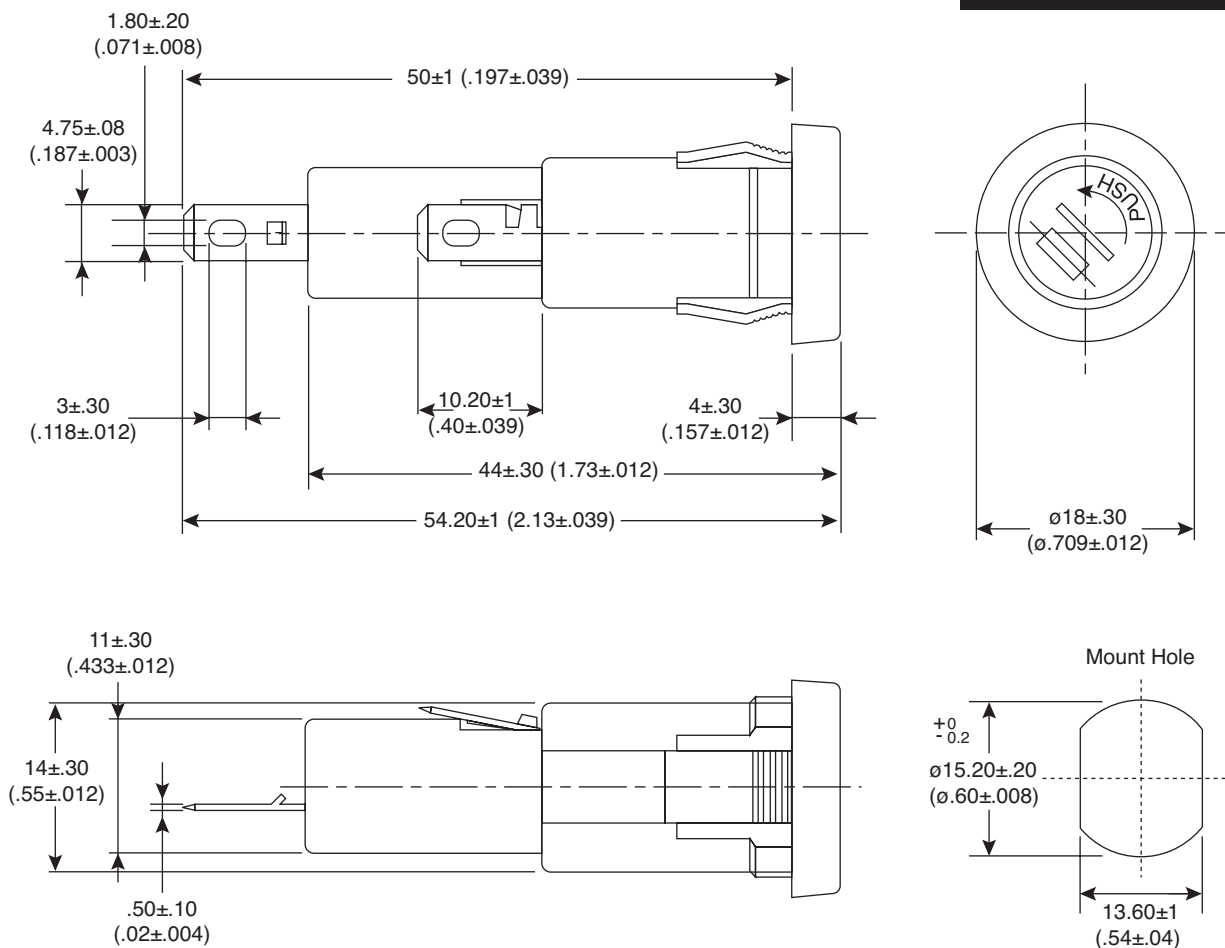
Dimensions: mm (in.)
