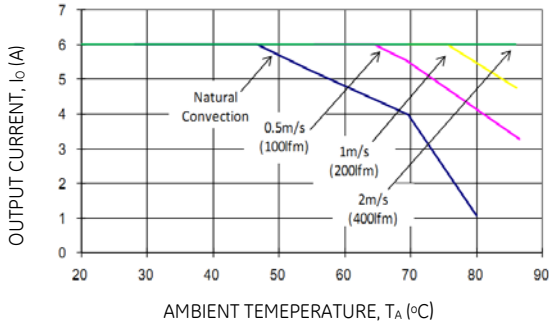
Figure 18. Output Current Derating for the Module with Heat plate; Airflow in the Transverse Direction from V out (-) to V out (+); V IN = 24V.
