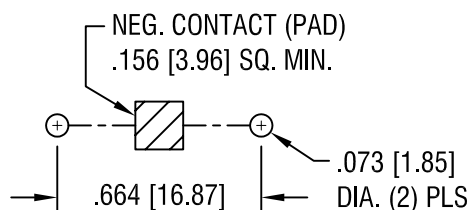
MOUNTING DETAIL
