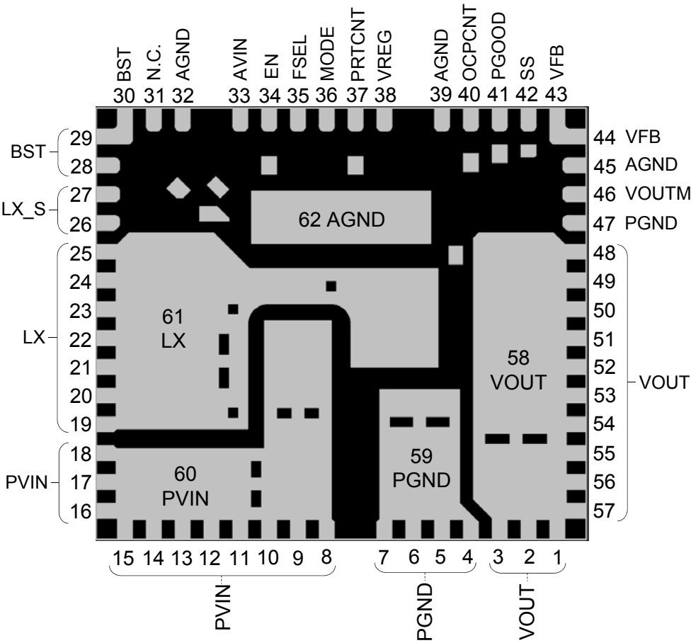
Bottom View
