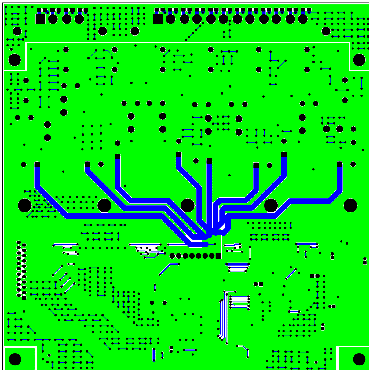
Figure 13. Bottomside Layer
