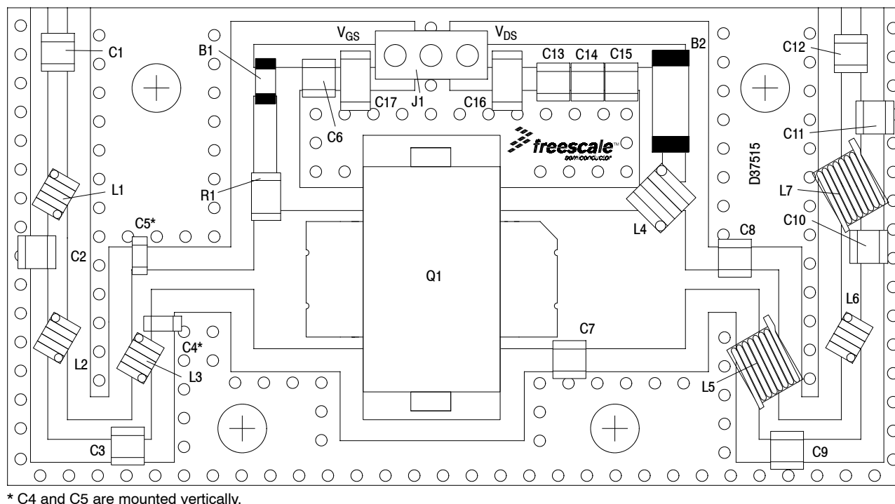
Figure 17. AFT05MS031NR1 UHF Broadband Reference Circuit Component Layout — 380-450 MHz
