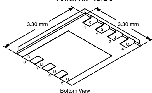
PowerPAK® 1212-8
