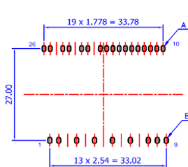
LAND PATTERN RECOMMENDATIONS
