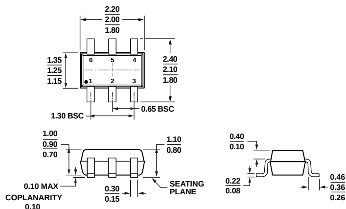
Figure 31. 6-Lead Thin Shrink Small Outline Transistor Package [SC70] (KS-6)
