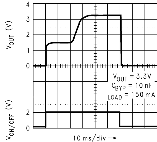
Figure 38. Turn-On Time
