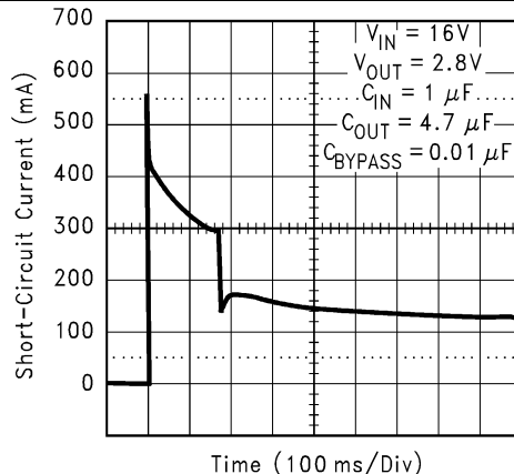
Figure 26. Short-Circuit Current
