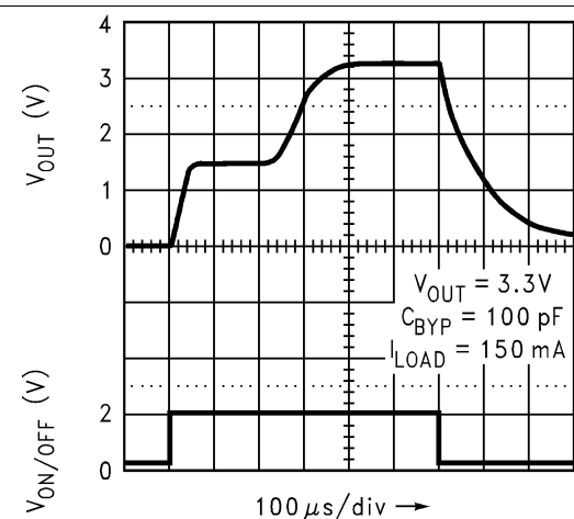
Figure 36. Turn-On Time
