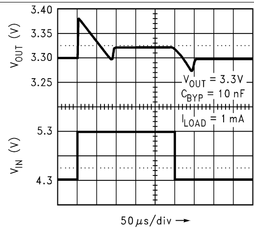
Figure 33. Line Transient Response
