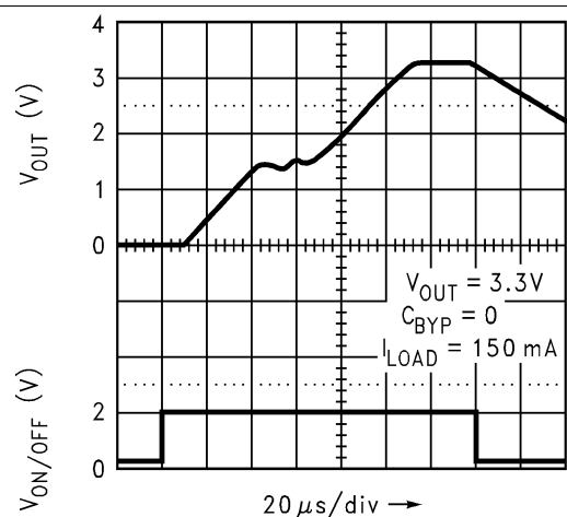
Figure 35. Turn-On Time
