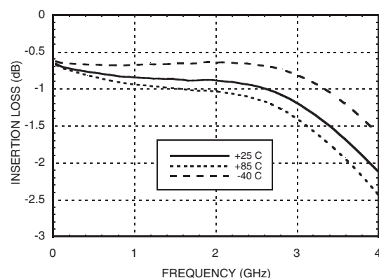
Insertion Loss [1]
