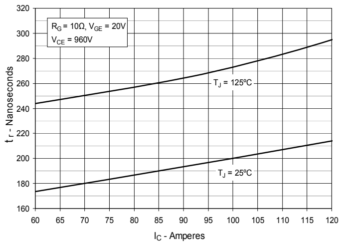
Fig. 15. Resistive Turn-on Rise Time vs. Collector Current
