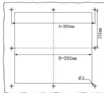
PANEL CUTOUT
