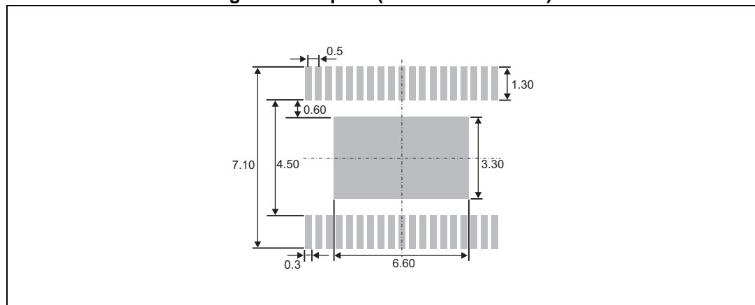
Figure 5. footprint (dimensions in mm)
