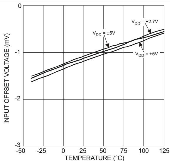
Figure 1 Input Offset Voltage vs. Temperature
