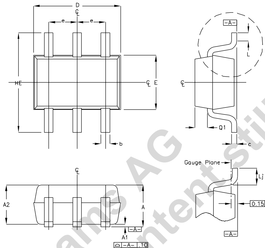
Figure 20. SC70-6 Package
