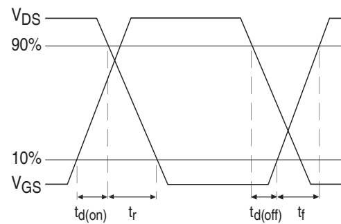
Fig 15b. Switching Time Waveforms www.irf.com
