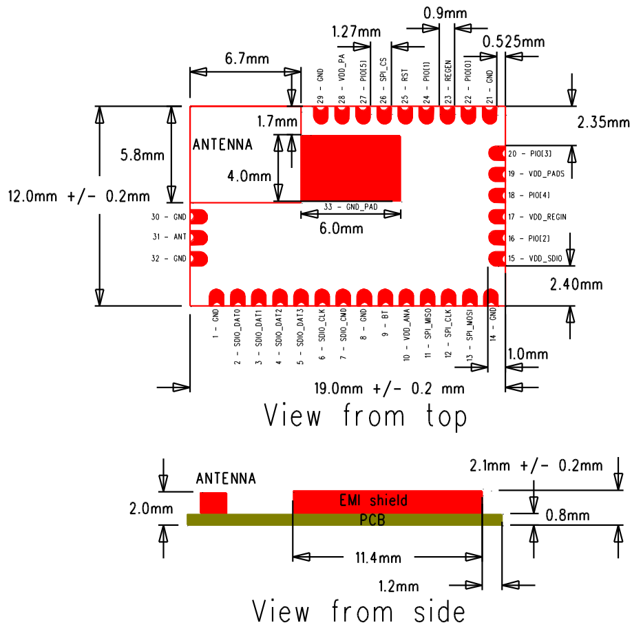
Figure 11: Physical dimensions
