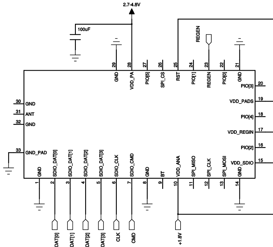
Figure 10: An example application circuit with SDIO host connection, 1.8V level host logic and a separate power amplifier supply, RST hard wired to the core supply and REGEN pad used to power off and reset the module (Note: with N-variant ANT-pad and associated grounds would also be connected)
