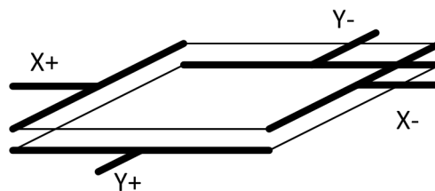
Figure 4 Touchscreen Plates X and Y
