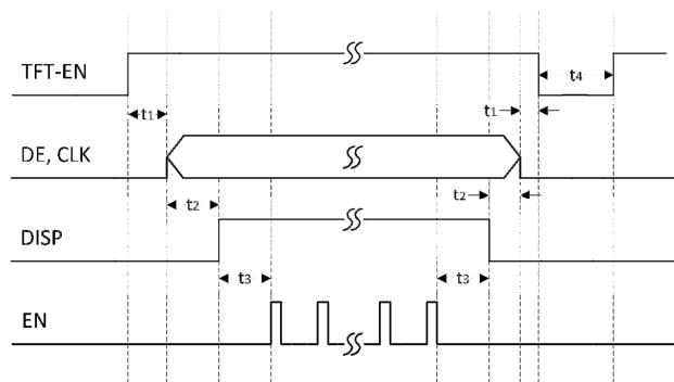
Figure 1 Power-Up Sequence
