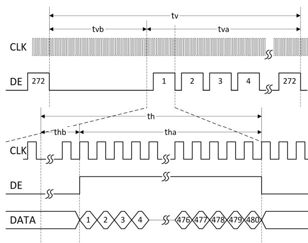
Figure 2 Video Timing
