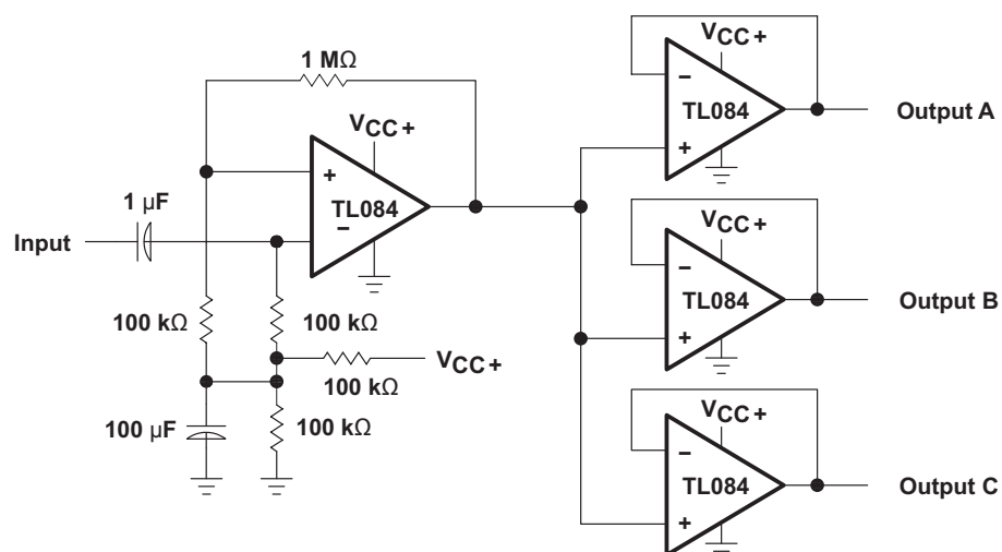
Figure 25. Audio-Distribution Amplifier
