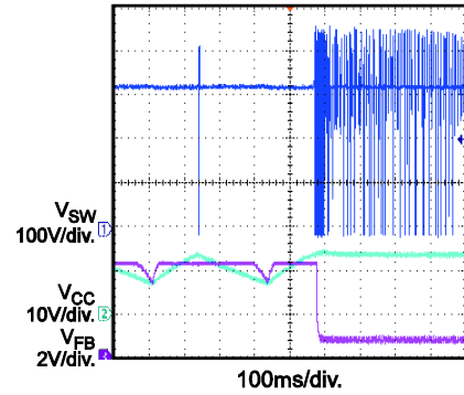
SCP Recovery 230Vac, No Load
