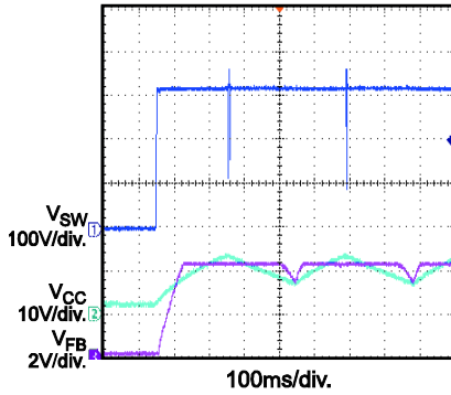
SCP Startup 230Vac, Full Load
