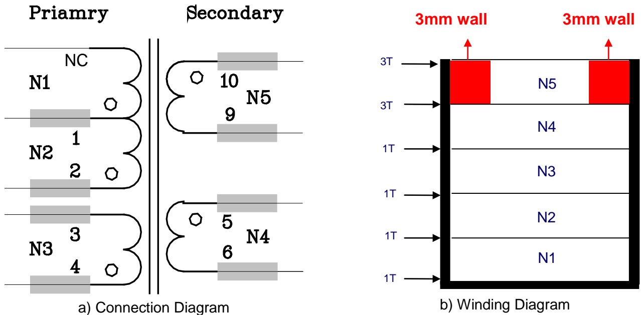
Figure 13: Transformer Structure
