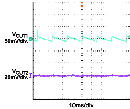
Output Ripple 230Vac, No Load
