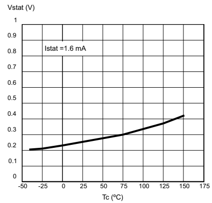
Figure 19. Status low output voltage
