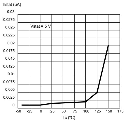
Figure 18. Status leakage current
