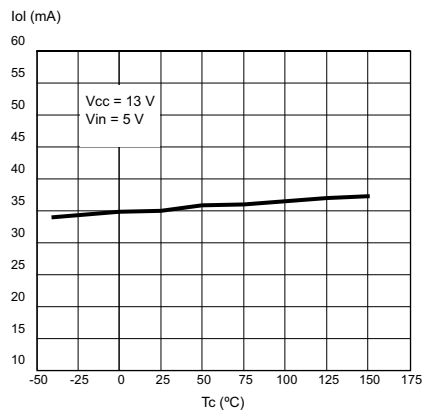
Figure 20. Openload on-state detection threshold
