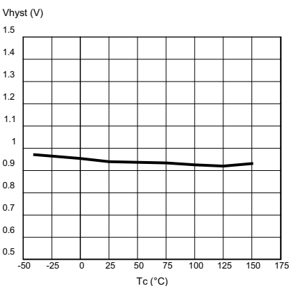
Figure 11. Input hysteresis voltage
