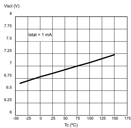
Figure 22. Status clamp voltage
