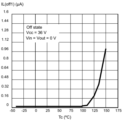
Figure 6. Off-state output current
