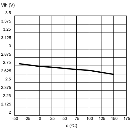
Figure 9. Input high level voltage
