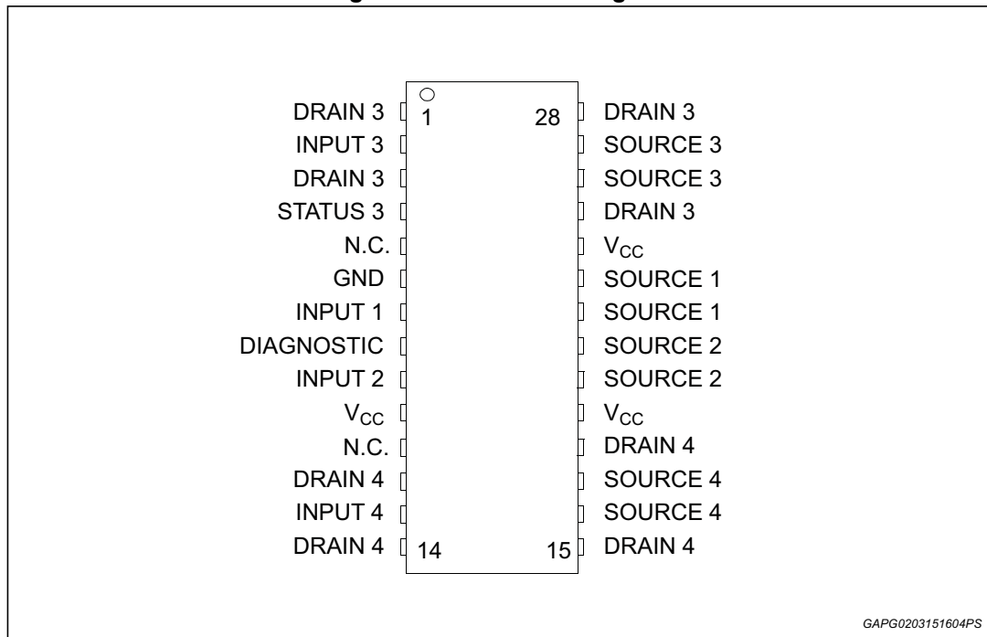
Figure 2. Connection diagram
