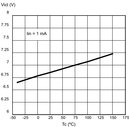
Figure 7. Input clamp voltage
