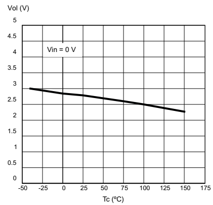
Figure 21. Openload off-state voltage detection threshold
