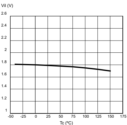
Figure 10. Input low level voltage
