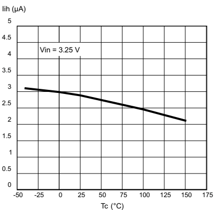
Figure 8. High level input current
