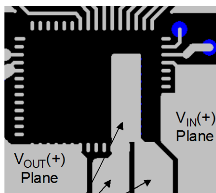
Local Ground Plane Slit separating input local ground from output local ground
