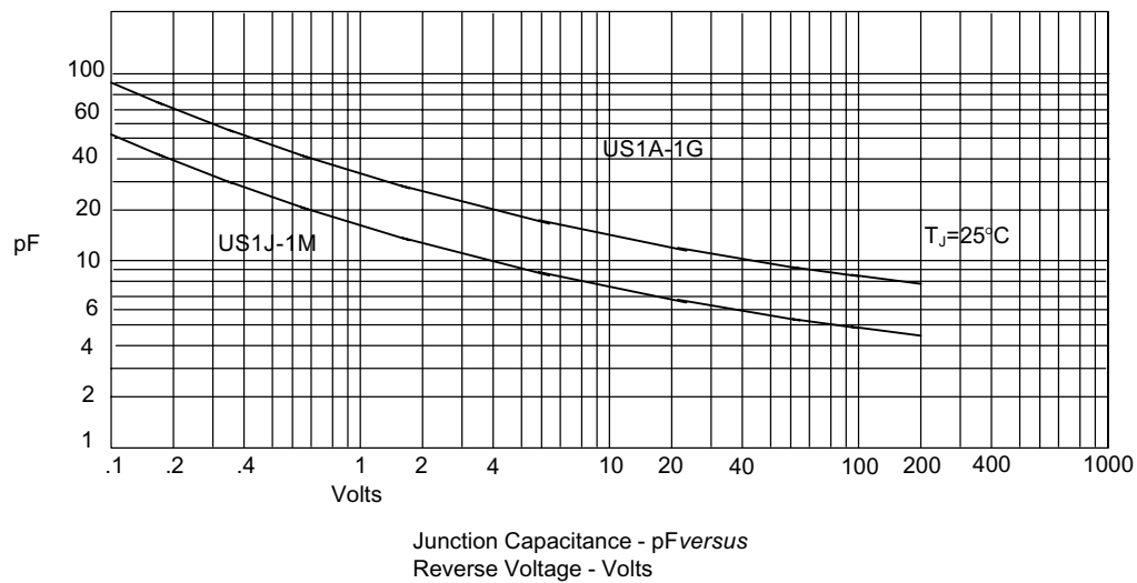
Figure 4 Junction Capacitance
