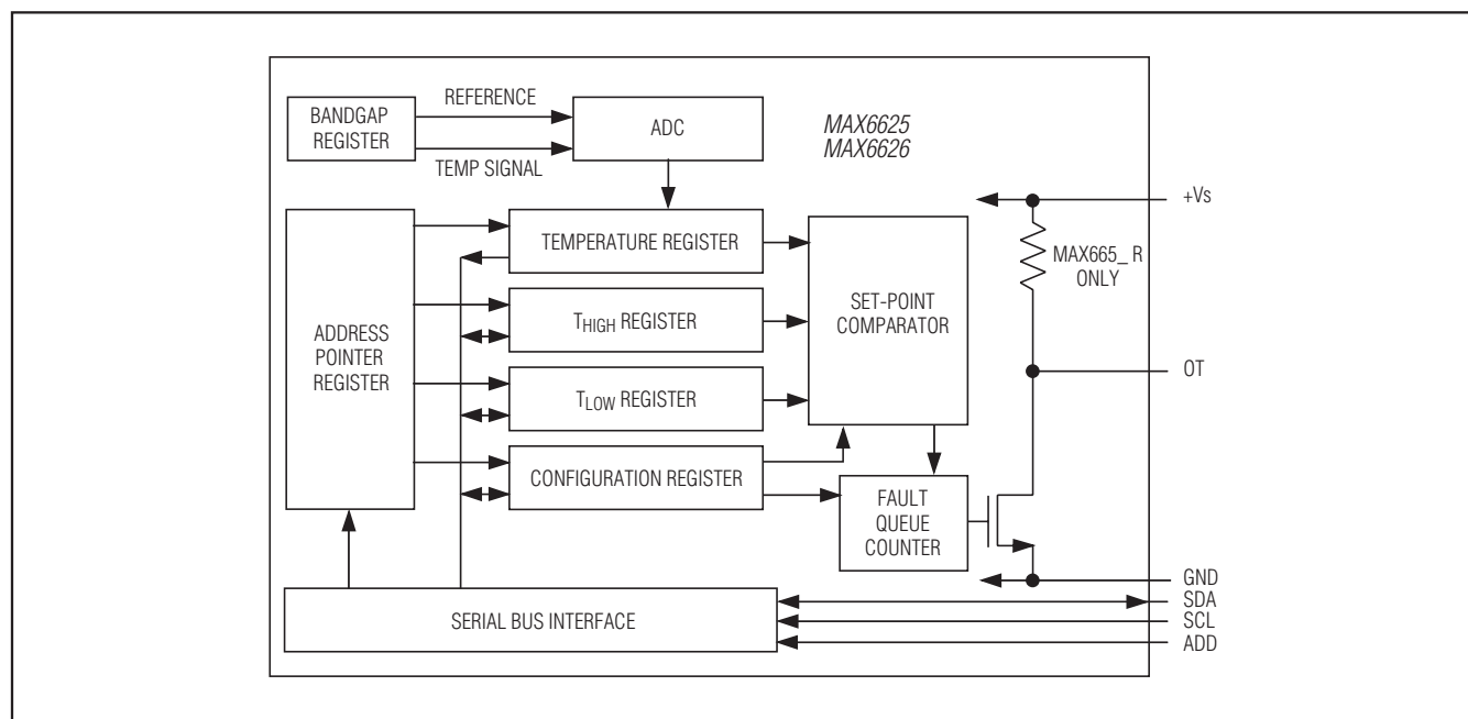
Figure 2. Functional Diagram
